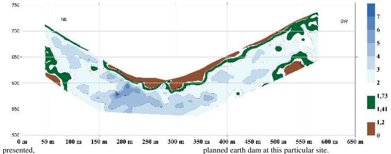
Figure 15. Dam case study 2: Generalized presentation of geotechnical significance based on Q-rock factor equal to V_P to V_S ratio.
