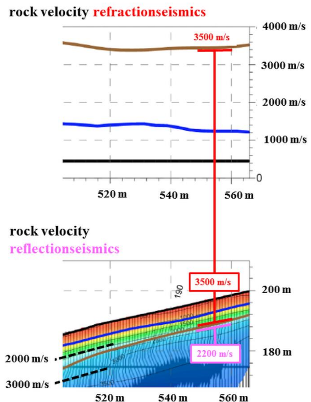
Figure 4. Sequential Hybridseismics delivers ambiguous velocity fields – velocity values derived from refraction tomography and values derived from reflection seismic processing occupying the same underground coordinate and violating rules of spatial congruency and reciprocal calibration. The velocity difference at one subsoil coordinate differs by 1300 ms -1 ;
