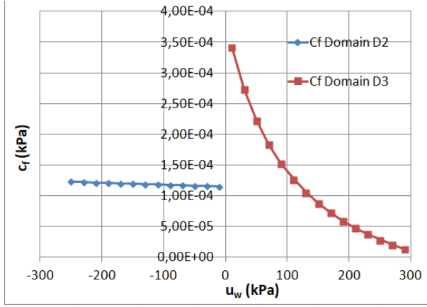
Figure 2. Evolution of the compression coefficient of the interstitial fluid c_f (water + occluded air) calculated with S_{re} = 0.96 , S_{air} = 0.85 : for domain D2 (blue curve) with S_r varying between 0.90 and 0.96; for the domain D3 (red curve) with S_r varying between 0.96 and 0.995
