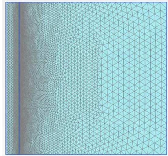
Figure 4. Plaxis mesh used for the Finite Element calculation.
