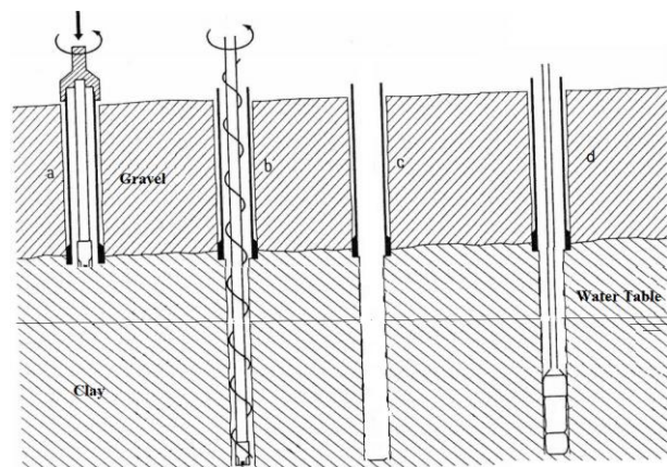
Figure 1. The main steps in carrying out the pressuremeter test
