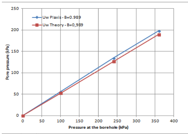
Figure 5. Large Deformation - Comparison of pore pressures at the borehole versus total the total stress applied, B = 0.989 .
