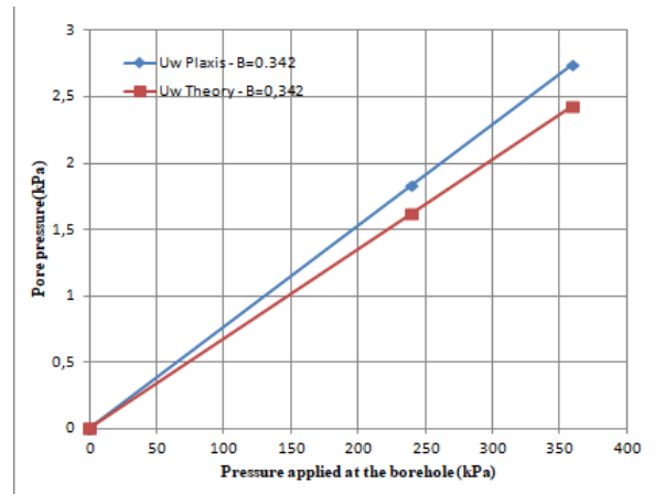
Figure 8. Large Deformation - Comparison of pore pressures at the borehole versus total the total stress applied, B = 0.342 .
