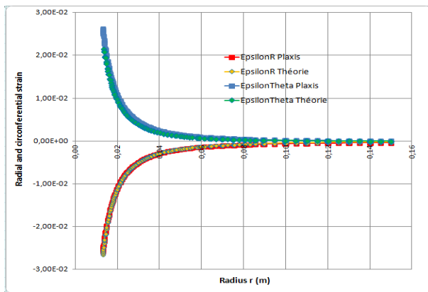
Figure 6. Large Deformation - Comparison of displacements at the borehole versus total the total stress applied, B = 0.989 .
