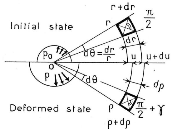
Figure 3. Elemental deformation condition in the horizontal plane by Baguelin [12].
