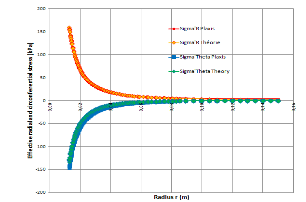
Figure 9. Large Deformation - Comparison of displacements at the borehole versus total the total stress applied, B = 0.342 .
