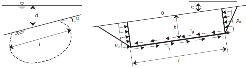
Figure 10: (a) Zone of elevated pore pressures, (b) Slope failure mechanism (after Puzrin et al. , 2004)
