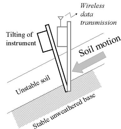
Fig. 15 Working mechanism of tilting sensor.
