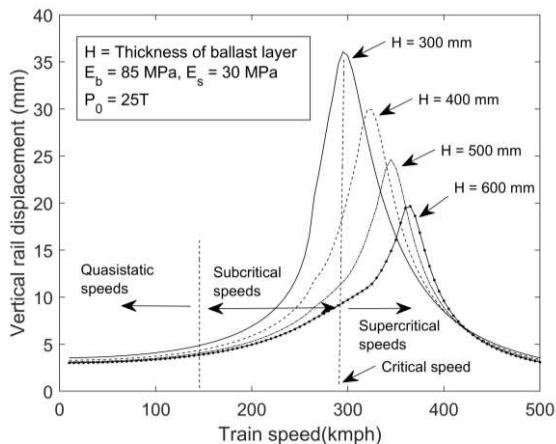
Figure 4. Dynamic vertical displacement response of rail at different train speeds
