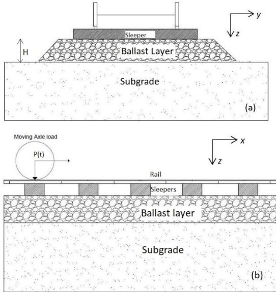
Figure 1 (a) Cross-sectional view and (b) longitudinal view of railway track
