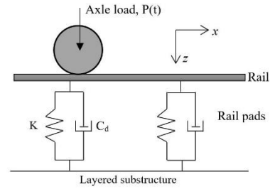
Figure 2. Rheological model of the superstructure of the railway track
