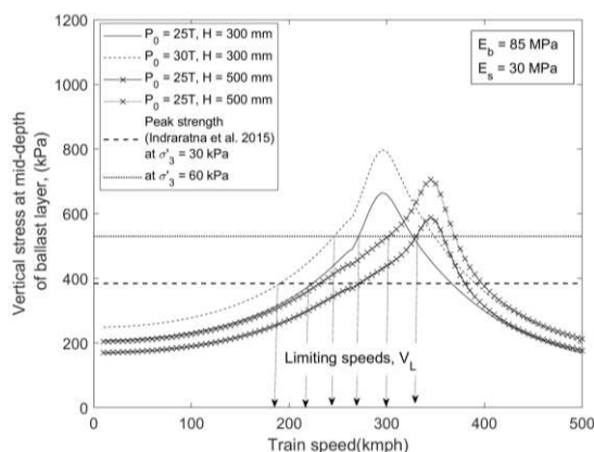
Figure 7. Comparison of dynamic stresses with peak static deviatoric strength of ballast at different train speeds, Peak strength data sourced from Indraratna et al. (2015)
