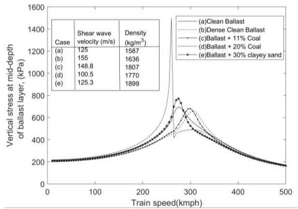
Figure 6. Effect of vertical stress at mid-depth of ballast layer for different ballast layer fouling. Shear wave velocity and density data sourced from Anbazhagan et al. (2011)
