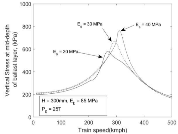
Figure 5. Dynamic vertical stress response in the mid-depth of the ballast layer at different train speeds
