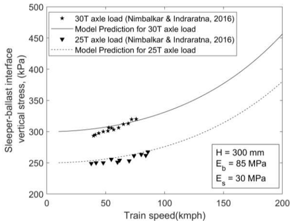
Figure 3. Dynamic sleeper-ballast interface vertical stress at different train speeds: model predictions compared with field measurement from Nimbalkar and Indraratna (2016)
