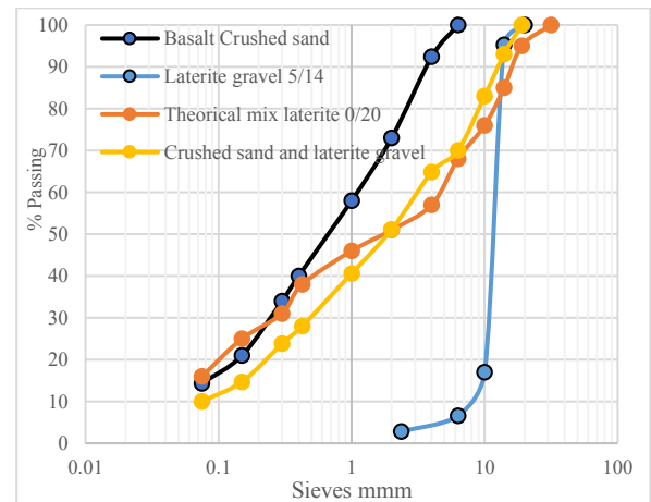
Figure 3: Theoretical mixtures F1 and F2
