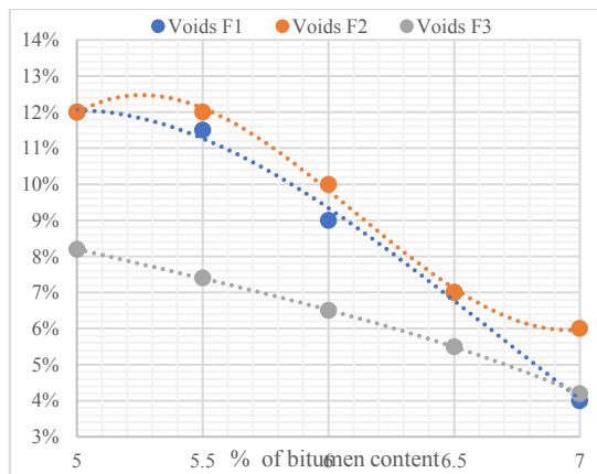
Figure 4. Evolution of voids in the three mixes
