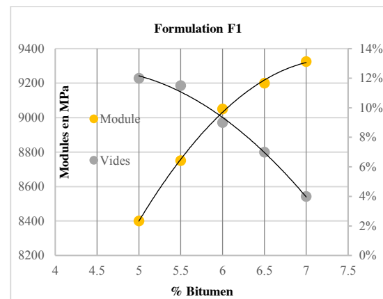
Figure 6 : Intersection of the module and voids in mineral
