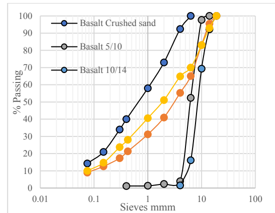
Figure 2: Theoretical mixtures F2 and F3
