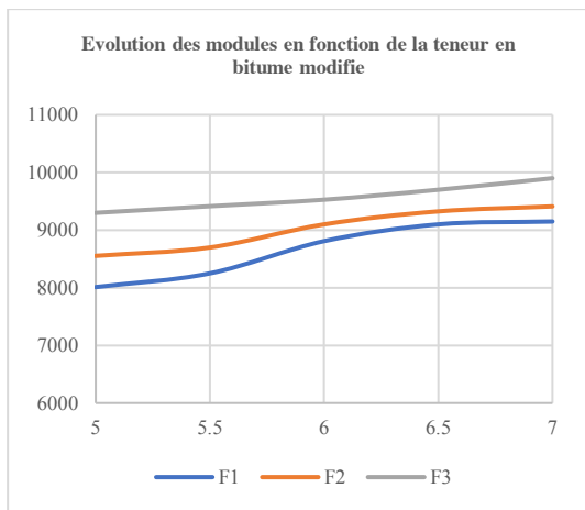
Figure 9 Variation in modules in relation to bitumen content in F3 bitumen content in F1, F2 and F3.
