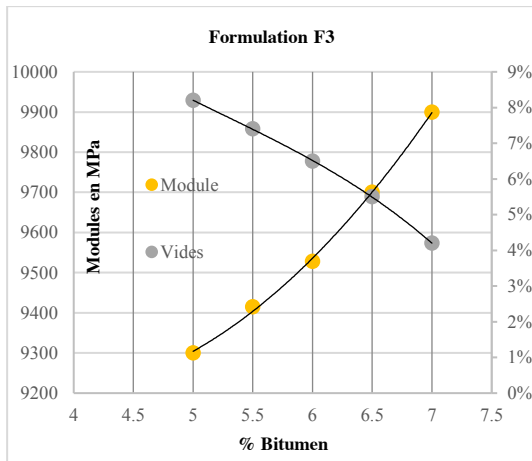
Figure 8 : Intersection of the module and voids in mineral
