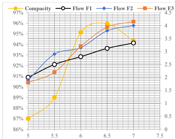
Figure 4. Evolution of voids in the three mixes
