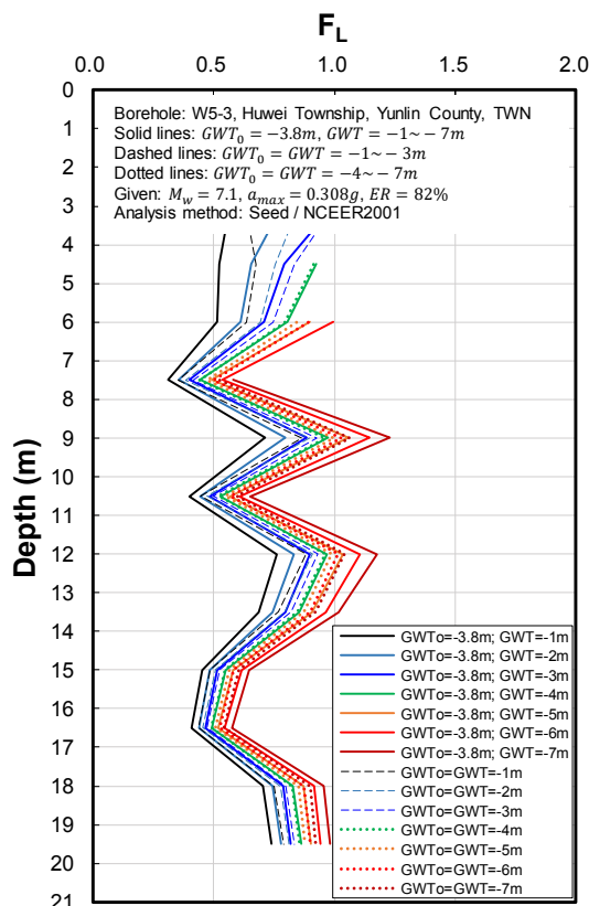
Figure 3. Computed F_L \sim Depth profiles at Borehole W5-3, a sandy deposit in Huwei Township, Yunlin County, Taiwan, with or without 1-GW assumption.
