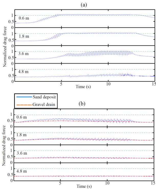
Figure 4. Time histories of vertical fluid drag force normalized by the average particle weight at selected depths inside (a) the loose deposit, and (b) the deposit with the drain
