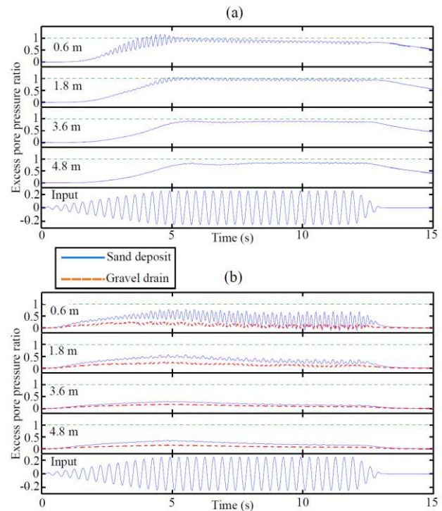
Figure 3. Time histories of excess pore water pressure at selected depth locations inside (a) the loose deposit, and (b) the deposit with the drain
