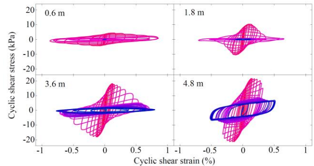
Figure 7. Shear stress-strain loops at selected depths (the loose deposit)
