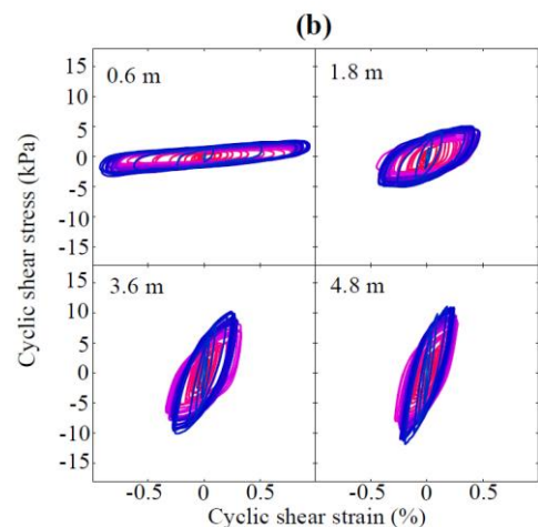
Figure 8. Shear stress-strain loops at selected depths: (a) inside the gravel drain, and (b) within the surrounding sand.
