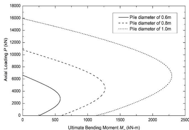
Figure 9. The axial loading vs. bending moment interaction diagrams for the project piles with various diameters (WIKI 2016)
