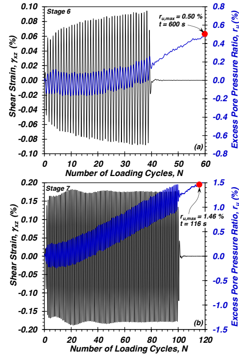
Figure 4. Shear strain and excess pore pressure ratio time histories for T-Rex loading and the 2PPT position at 2 m depth: (a) Stage 6, N = 40 , and (b) Stage 7, N = 100 .
