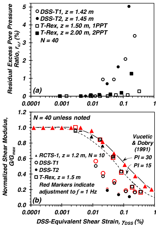
Figure 5. Comparison of in-situ and laboratory-derived variation of (a) residual excess pore pressure ratio, r_{ur} and (b) shear modulus reduction, G/G_{max} , with shear strain.
