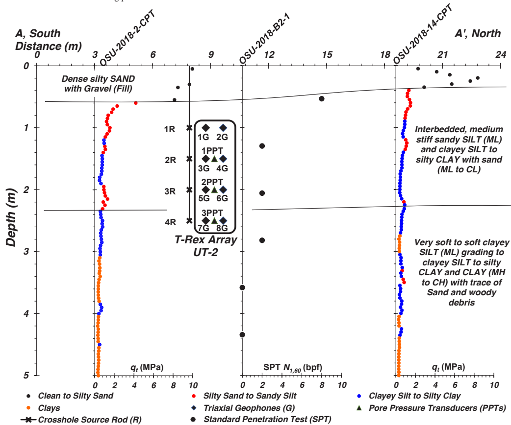
Figure 2. Subsurface conditions along Section A-A' in proximity to instrumented array UT-2, situated 10 m east (out of plane) of Section A-A'.
