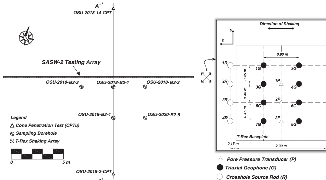
Figure 1. Site and exploration plan at test panel UT-2; inset figure presents the plan view of instruments within the T-Rex loading footprint. Section A-A' is shown in Figure 2.
