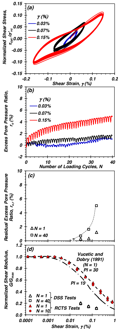
Figure 3. Cyclic response of selected specimens: (a) \tau_{cyc}/\sigma'_{vc} - \gamma hysteresis, and variation of: (b) r_u with N , (c) r_{ur} with \gamma for N = 1 and 40, and (d) G/G_{max} with \gamma and comparison to Vucetic and Dobry (1991).
