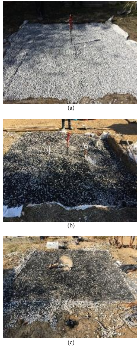
Figure 8. The three soil pits (of dimensions 3.2m x 3.2m x 0.5m) filled with rubber-gravel mixtures (RGM): (a) 0%, (b) 25% and (c) 75% rubber contents by volume.
