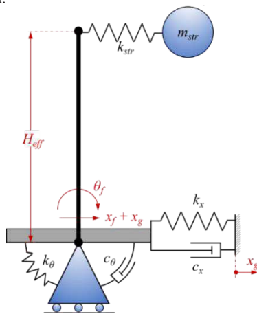
Figure 1. The mass-spring-dashpot model of a soil-shallow foundation-structure system adopted in the equivalent-linear analytical model (Tsang & Pitolakis 2019).
