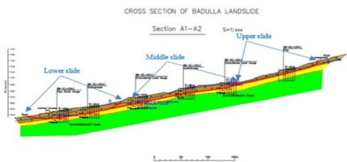
Figure 2. Long section along A1- A2 (JICA Report, 2015)
