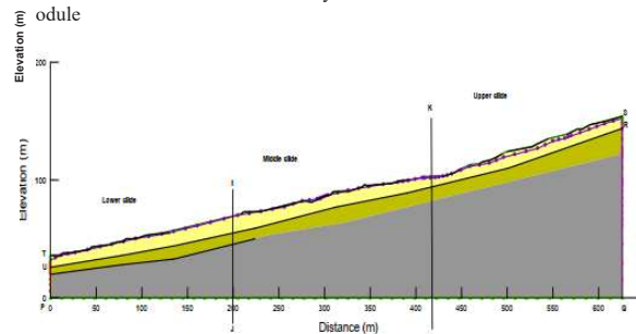
Figure 3. Long section idealized in SLOPE/W and SEEP/W
