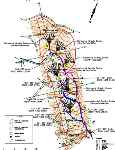
Figure 6. Plan view of the proposed drainage improvement
