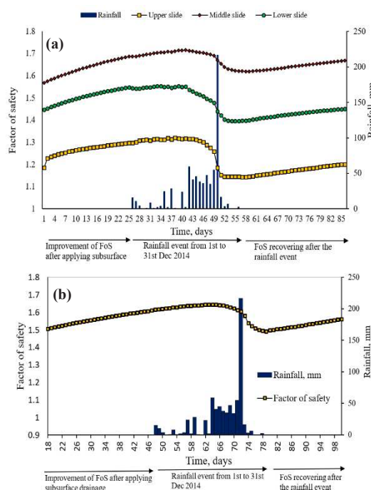
Figure 9. Variation of factor of safety with response to the critical rainfall event simulated : (a) For three individual slides, (b) Composite slide
