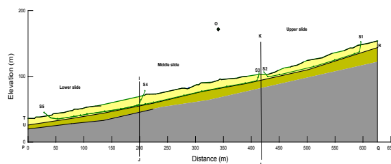
Figure 5. The slip surfaces of each slide are fully defined in SLOPE/W module
