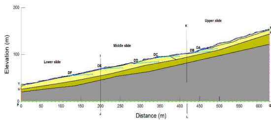
Figure 7. Drains simulated in the section A1 - A2
