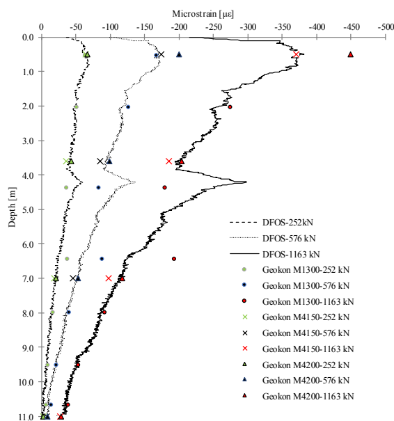
Figure 12. Strain distribution measured by DFOS and VWSG along the pile shaft at selected load values.
