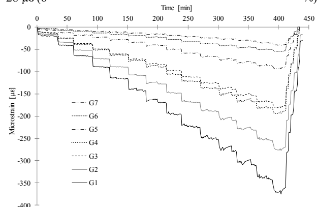
Figure 6. Strain measured by retrievable extensometers.
