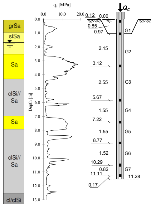
Figure 1. CPT sounding, soil and pile profile.
