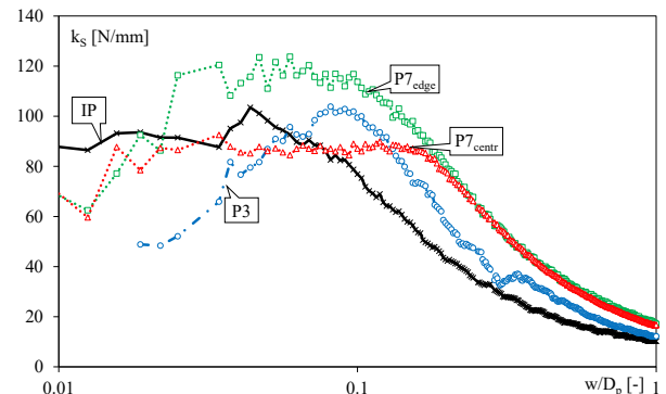
Figure 13. Pile shaft stiffness k_s vs. the normalized pile settlement w/D_p . Model scale.
