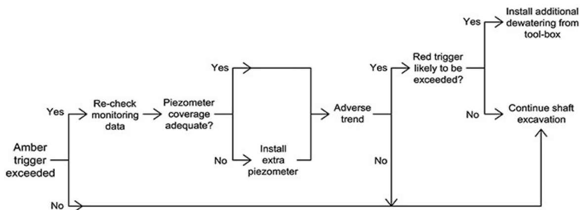
Figure 12. Crossrail Blomfield box – OM groundwater control chart
