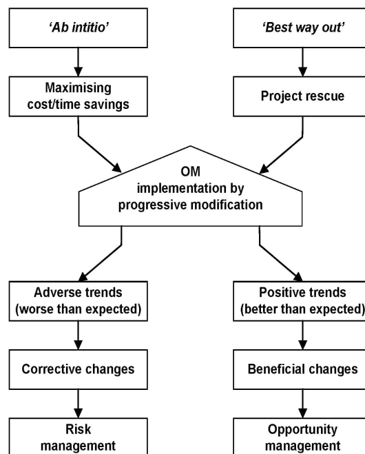
Figure 31. Progressive Modification, all OM categories can be addressed.
