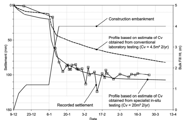
Figure 5. Dearne Town embankment. Construction, observed and calculated consolidation settlement vs time curves.
