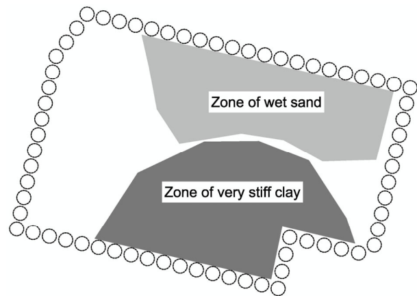
Figure 15. Crossrail Blomfield box, configuration of clay and sand layers at 73 m ATD
