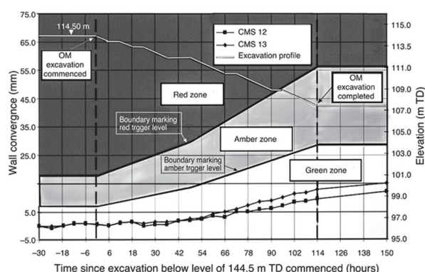
Figure 30. Example of OM traffic light control zones (after Powderham and O'Brien, 2020)
