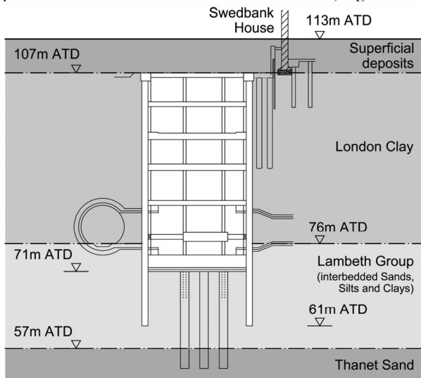
Figure 6. Crossrail Blomfield box and simplified geological profile.
