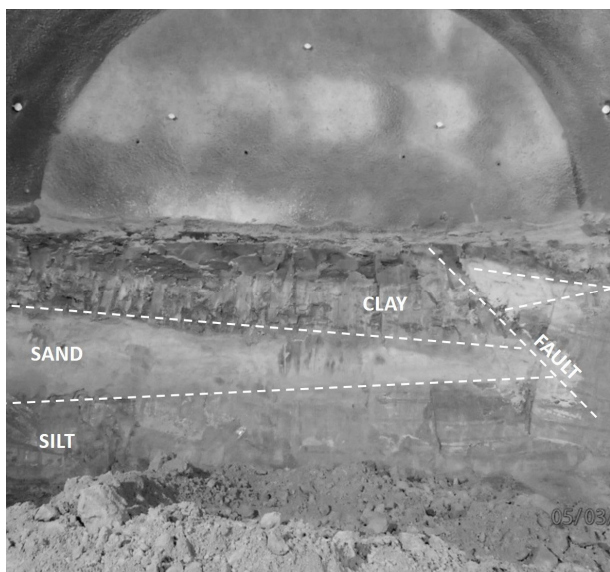
Figure 9. Exposure of Lambeth Group at invert of SCL tunnel. (Note: Fault at right-hand side and interbedded sand/clay/silt layers)
