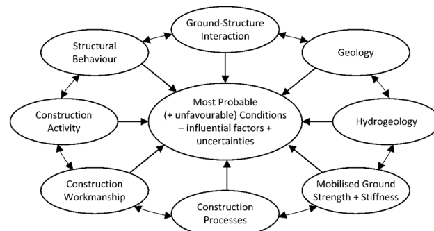
Figure 32. Observational Method, most probable and unfavourable conditions - some influential factors.
