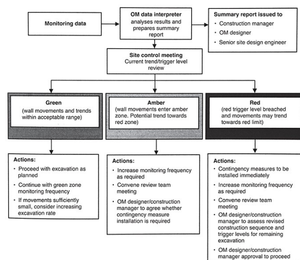
Figure 29. Example of OM site control flow chart (after Powderham and O’Brien, 2020).
