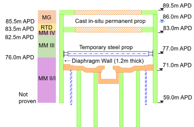
Figure 19. Typical section at BTWP.
