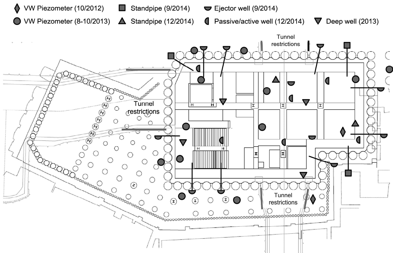
Figure 16. Crossrail Blomfield box, final layout of groundwater monitoring and wells (note slit trenches not shown for clarity).
