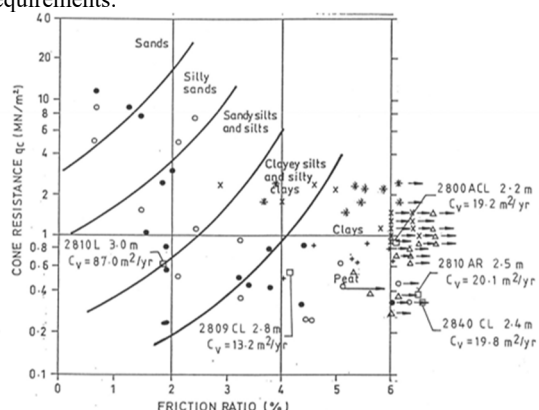
Figure 2. Deame Town embankment, CPT classification chart
