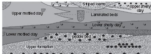
Figure 8. Potential variability of Lambeth Group (after CIRIA C583).
