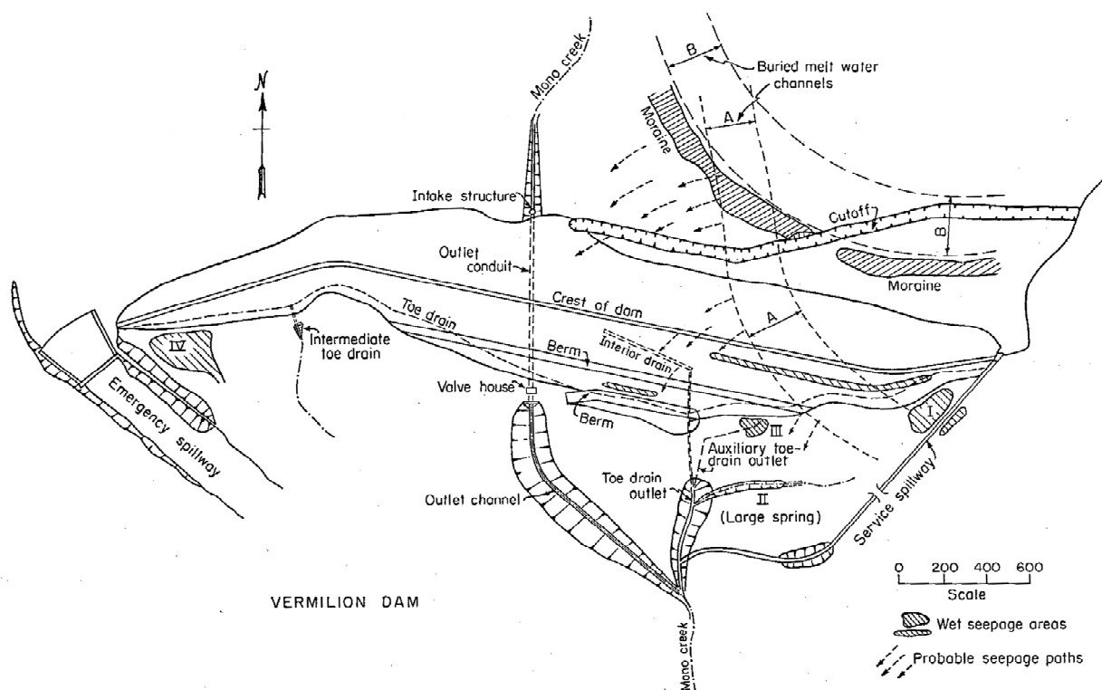
Figure 1. Plan of Vermillion Dam. In Areas I to IV water came out of the ground while the reservoir was being filled for the first time (after Terzaghi, 1961).
