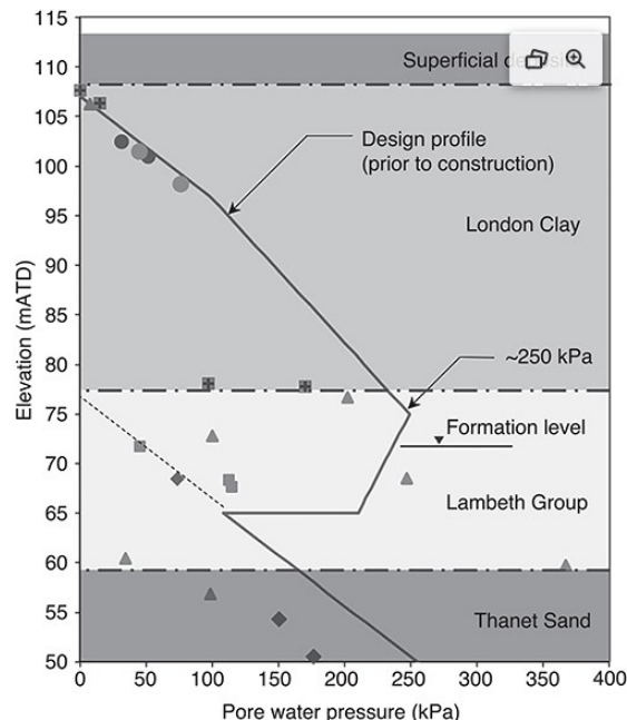
Figure 7. Crossrail Blomfield Box - groundwater pressures.
