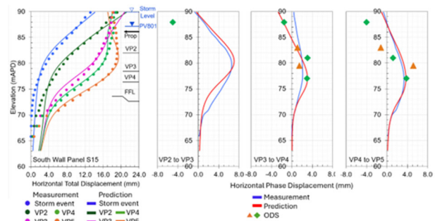
Figure 25. Results of near real time back analysis of WHRC, section A, South wall Panel S15 (ML1244-IPI801).
