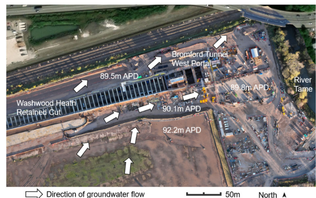
Figure 26. Direction of groundwater flow at BTWP and WHRC
