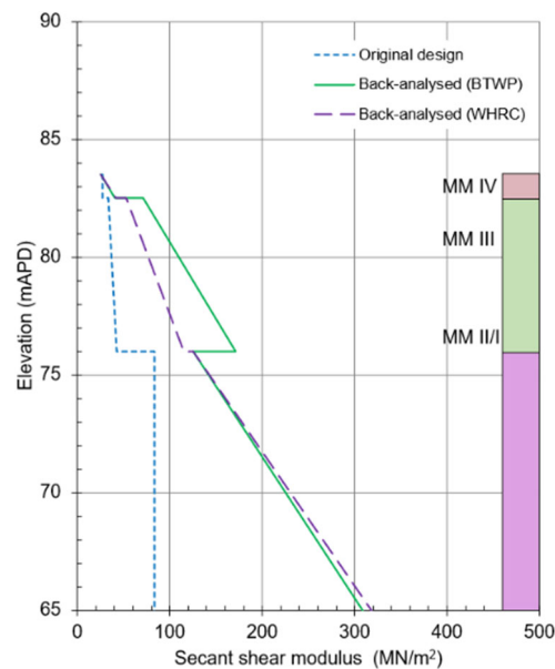
Figure 28. Comparison of secant shear modulus values of the Mercia Mudstone Group at BTWP and WHRC (panel S15).
