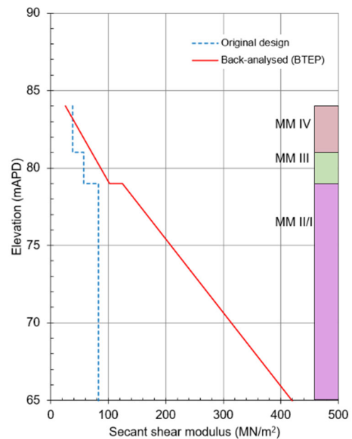
Figure 21. Comparison of secant shear modulus values of the Mercia Mudstone Group at BTEP
