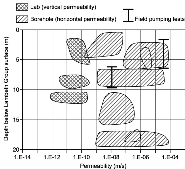
Figure 10. Permeability test values for Lambeth Group (lab, borehole and pumping tests).
