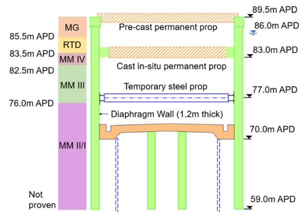
Figure 20. Typical section at WHRC (Section A).
