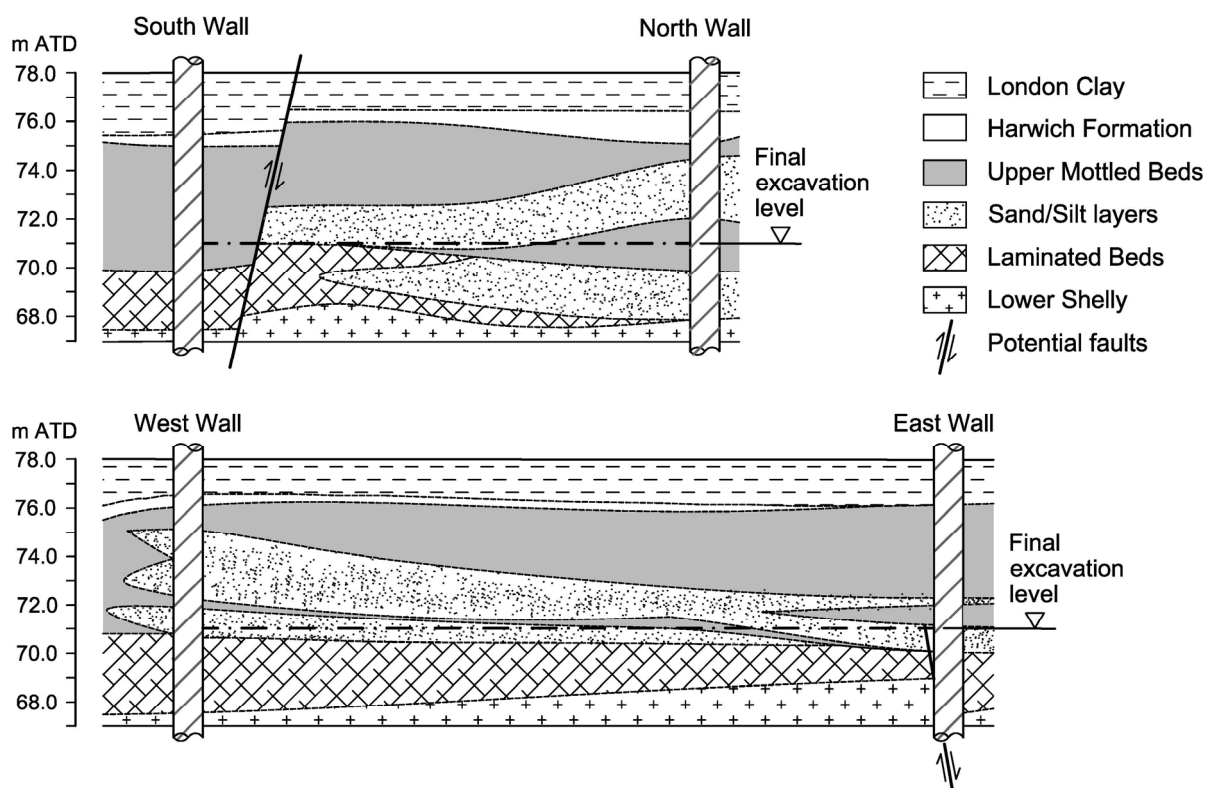
Figure 17. Crossrail Blomfield box – logged profile through Lambeth Group.
