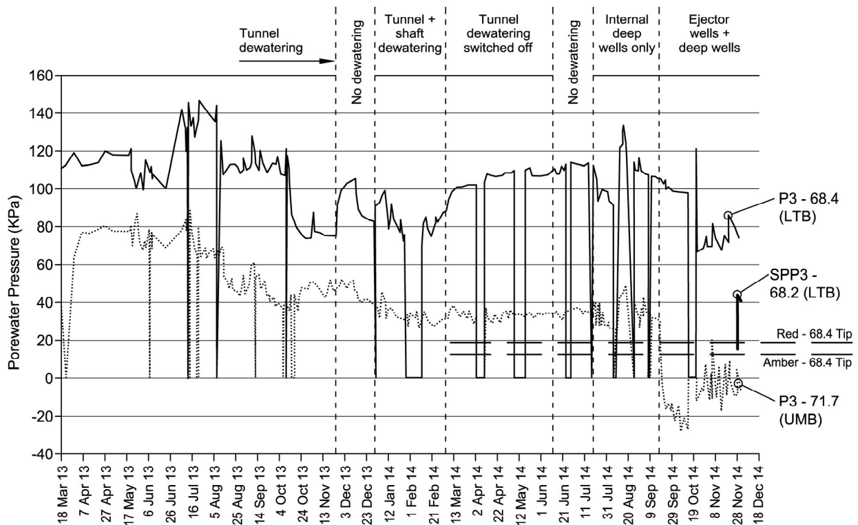
Figure 13. Crossrail Blomfield box, observed groundwater pressures, inside box, up to November 2014
