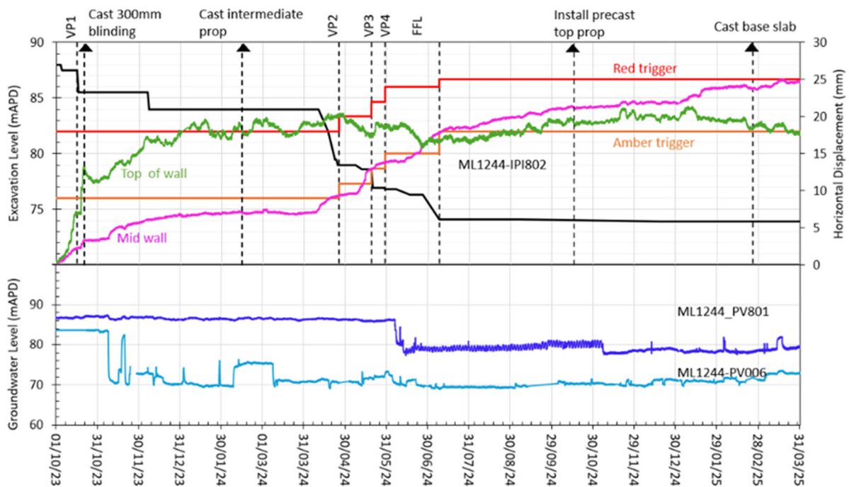
Figure 27. Progression of wall displacement and groundwater level over time at WHRC, section A, panel S15.
