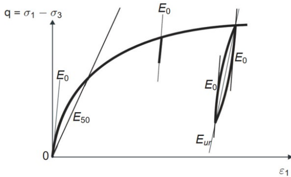
(b) Non-linear and hysteretic ground behaviour
