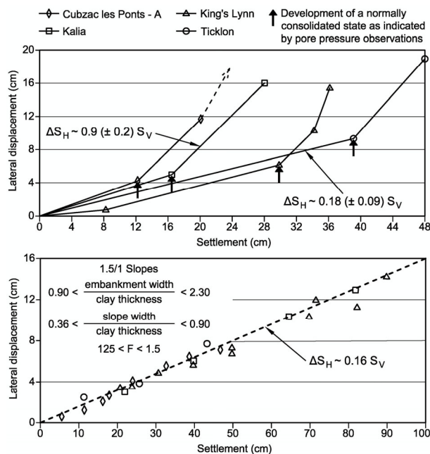
Figure 3. Case history observations of lateral displacement and settlement for embankments constructed on soft clay (after Tavernas & LeRoueil, 1980)
