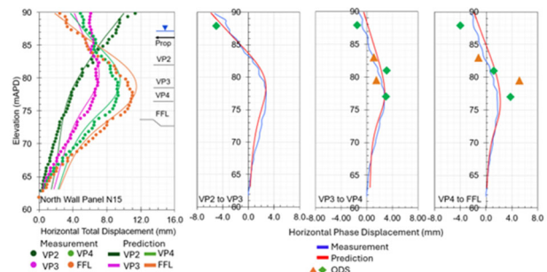
Figure 24. Results of near real time back analysis of WHRC, section A, North wall Panel N15 (ML1244-SAA802).
