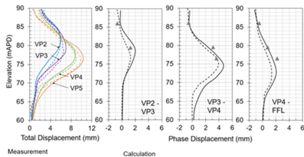
Figure 22. Measurement vs RTBA calculation – total and phase displacement at BTWP.
