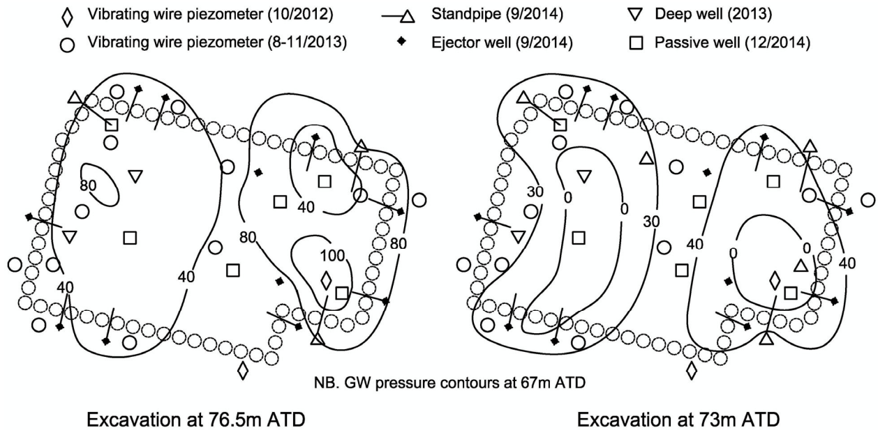
Figure 14. Crossrail Blomfield box, groundwater pressure contours, before and after final modifications to groundwater control systems
