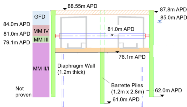
Figure 18. Typical section at BTEP (Eastern End).
