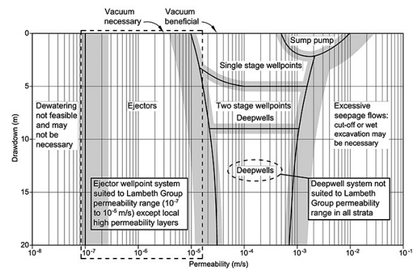
Figure 11. Permeability range for various pumped groundwater control techniques (modified after Preece, 2012).
