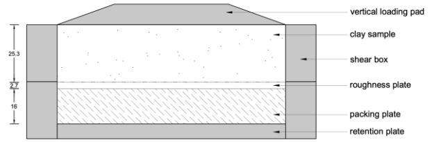
Figure 3. Cross-section of shear box for interface tests
