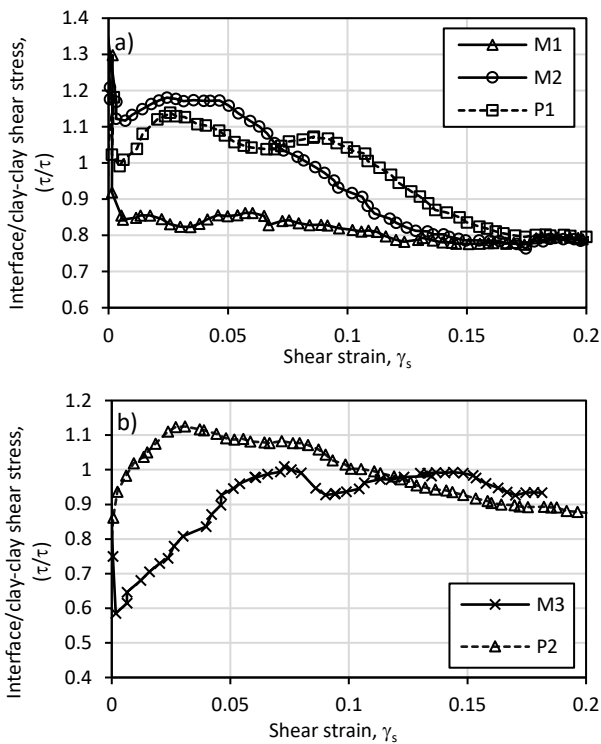
Figure 9. Normalised shear strength ( \tau/\tau ) against shear strain ( \gamma_s ) from the direct shear tests on the a) top layer, and b) bottom layer of Speswhite kaolin clay samples
