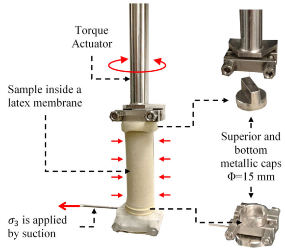
Figure 2. Experimental Set-up.
