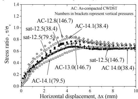
Figure 6. Stress ratio with horizontal displacement for saturated drained tests ( w_s = 12.5\% , solid symbols) and constant water content test at high S_r (open symbols).
