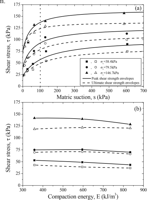
Figure 5. Shear strength envelopes for specimens compacted at (a) energy level of 596 \text{ kJ/m}^3 and (b) w = 12.8\sim 13\% (close and open symbols represent peak and ultimate states, respectively).
