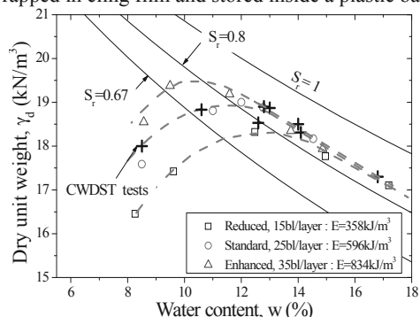
Figure 1. Compaction curves obtained for the silty sand soil.
