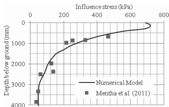
Figure 4. Validation of FEM model – dynamic case.
