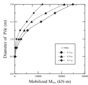
Figure 8 Maximum moments of piles varying pile diameter and PGAT
