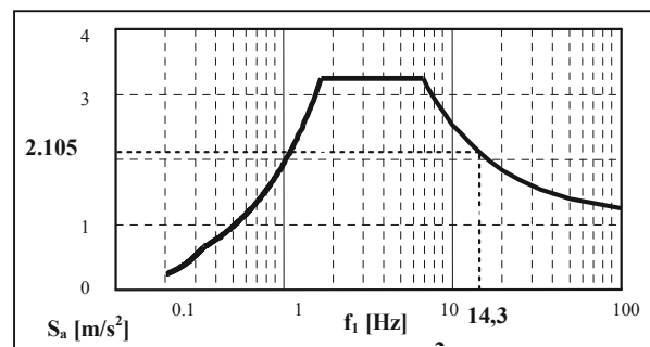
Figure 2. Elastic acceleration response spectrum medium stiff soil, 5% damping, a_g=1,1 \text{ m/s}^2 .
