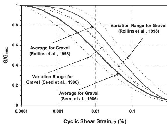
Figure 1. Typical G/G_{max} \sim \gamma relationships for gravels.
