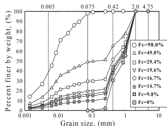
Fig.1: Grain size distribution curves of samples us
