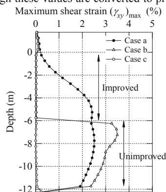
Figure 4. Shear strain distribution
