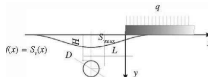
Figure 5. Mutual position of beam of semi-infinite length, and shallow utility tunnel with assigned support-line displacement f(x) .
