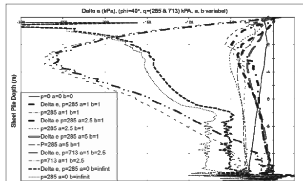
Figure 8 FE models results ( \varphi=40^\circ )
