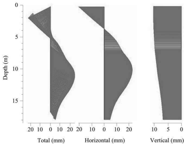
Figure 4. Displacement diagrams.
