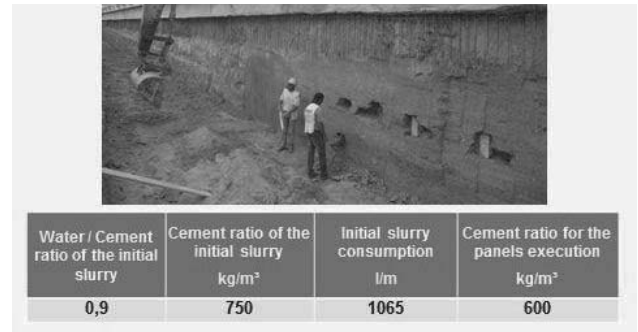
Figure 7. Adopted values for the CSM panels execution parameters.
