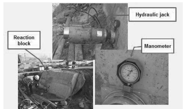
Figure 8. Permanent ground anchor suitability test.
