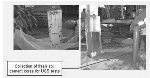
Figure 6. Collection of soil - cement fresh cores.
