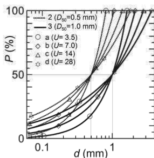
Figure 3. Grain size distributions of reconstituted LECA samples.
