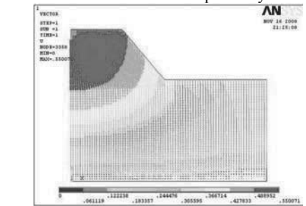
(a) computed displacement of unreinforced model
