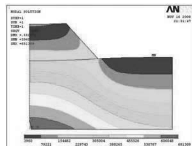
(a) stress contours of unreinforced model
