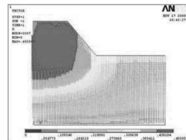
(b) computed displacement of reinforced model
