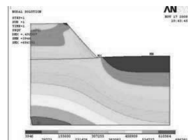
(b) stress contours of reinforced model
