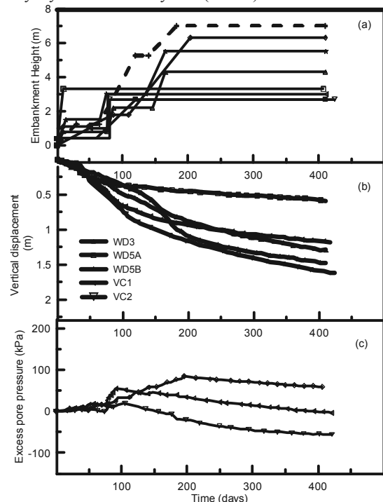
Figure 2. Embankment responses (a) staged construction, (b) settlements and (c) excess pore pressures
