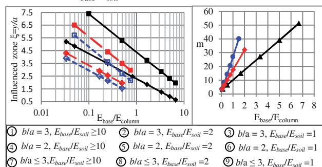
Figure 6. Stone column with compressible base -elastic solution
