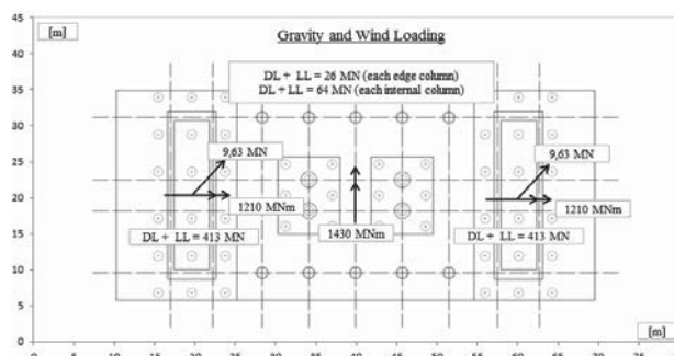
Figure 2 Piled-Raft foundation plan and loading.
