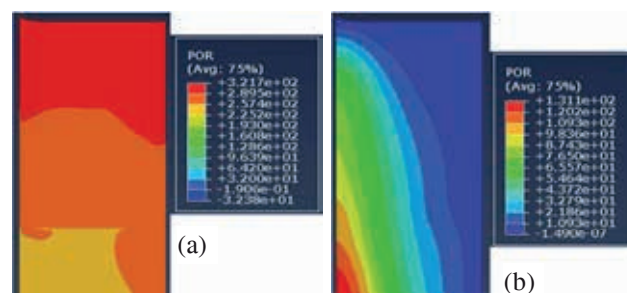
Figure 4. Radial effective stress distribution in numerical model: (a) EOID, (b) BOR after 13 days.
