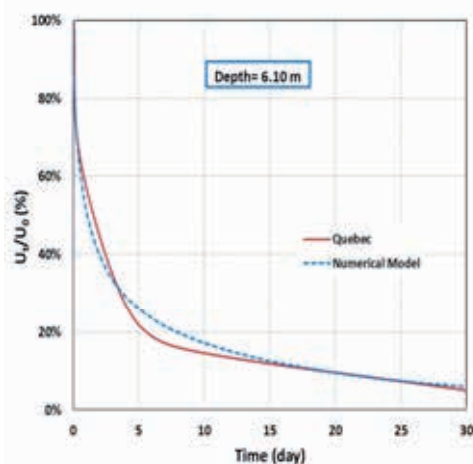
Figure 3. Dissipation of EPWP with time resulted from pile driving at depth 6.1 m.
