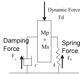
Figure 2: Model for the soil pile interaction in the pseudo-static model.
