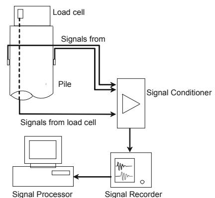
Figure 5: Testing electronic devices used for the pseudo-static load test.
