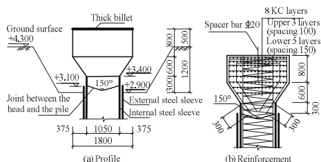
Figure 2 Design schematic diagrams of the test pile head for the Shanghai Center Tower project
