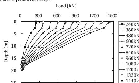
Figure 4. Axial force distribution for 20m-long single pile.
