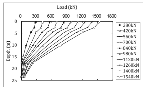
Figure 5. Axial force distribution for 24m-long single pile.
