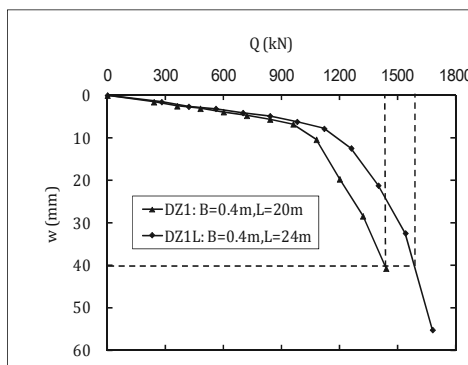
Figure 3. Load settlement curves for single pile tests.
