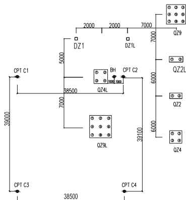
Figure 1. Layout plan of test piles and pile groups ( all dimensions in millimeters).
