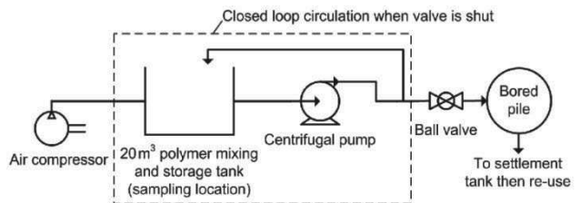
Figure 4. Schematic diagram of recirculation/delivery system.
