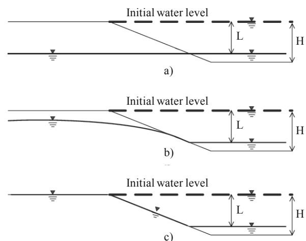
Figure 1. Water drawdown modes: a) Fully slow drawdown, b) Transient drawdown, c) Fully rapid drawdown (Berilgen 2007).
