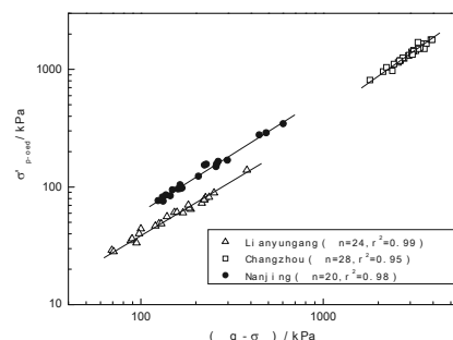
Figure 2. The relationship between preconsolidation pressure measured in oedometer test and net tip resistance
