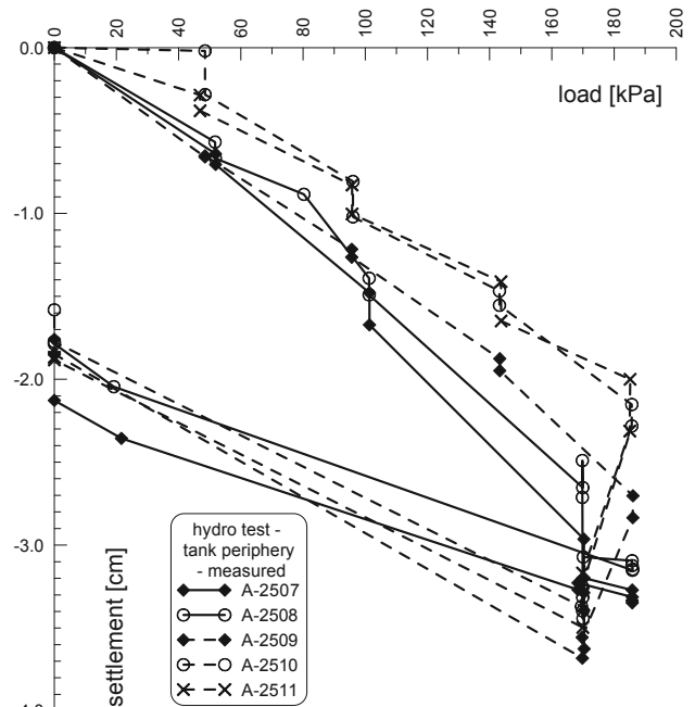
Figure 7. Total settlements of tank perimeters during hydro tests performed on all five tanks
