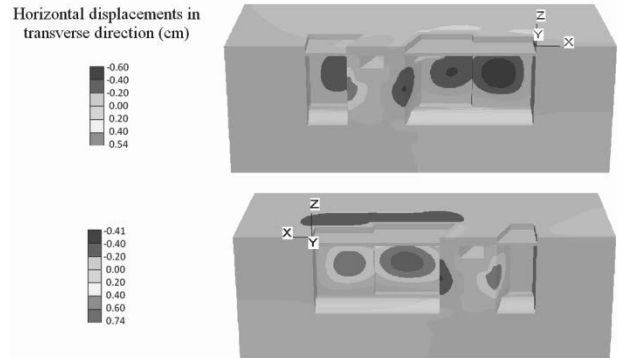
Figure 7. Horizontal displacements in transverse direction (stage c)
