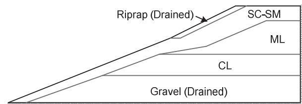
Figure 3. Cross-section of Walter Bouldin Dam
