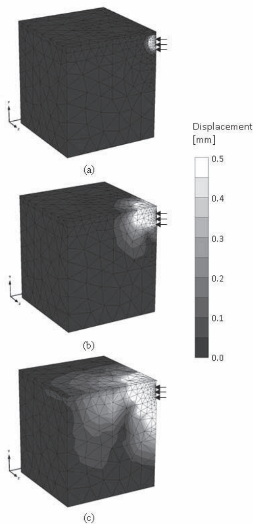
Figure 3. Displacements produced by the pressure wave propagation at different times after the blasting: (a) 0,01s; (b) 0,03s; (c) 0,06s.
