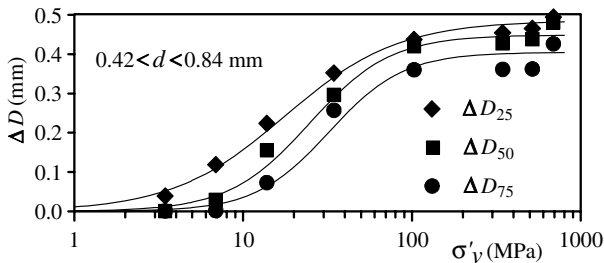
Figure 10. Progress of the changes \Delta D of characteristic diameters as a function of the applied stress \sigma'_v for angular glass (1-D tests). Data from Hagerty et al., 1993.
