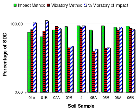
Figure 1. Comparison of Compaction Results for all Soils
