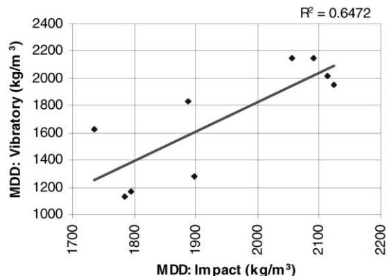
Figure 3. Correlation Between MDD (Vibratory Compaction) and MDD (Impact Compaction) for all Soils.
