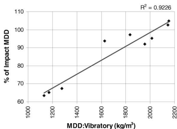
Figure 2. Correlation Between Percentage of MDD (Impact Compaction) and MDD (Vibratory Compaction) for all Soils.
