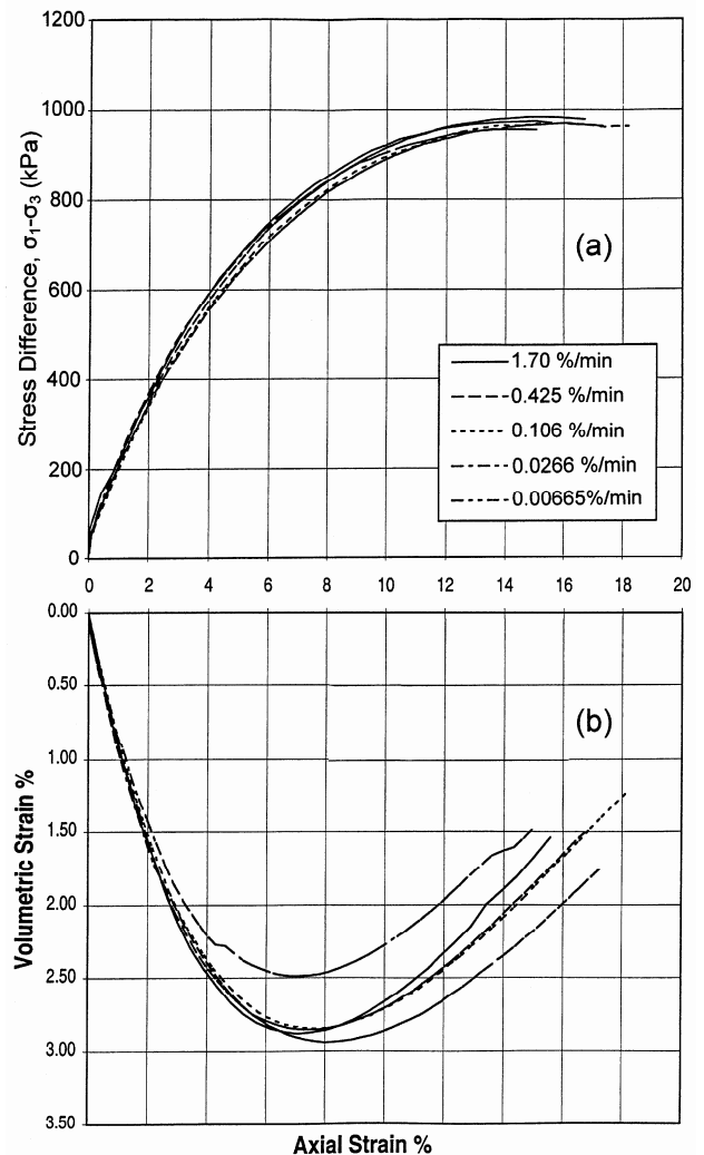
Figure 1. Comparison of (a) stress-strain and (b) volume change relations for drained triaxial compression tests on crushed coral sand performed with five different strain rates.
