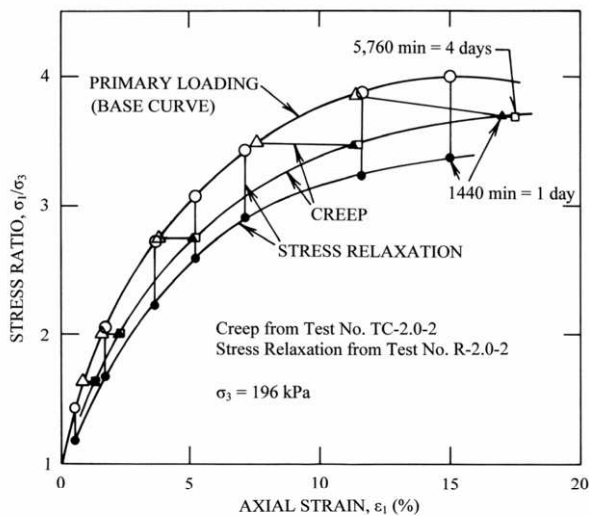
Figure 5. Comparison of creep and stress relaxation experiments performed in two triaxial compression tests on Antelope Valley sand.
