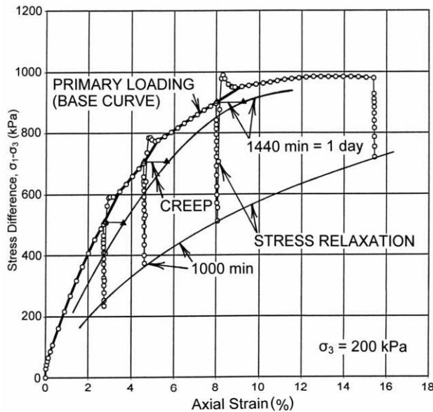
Figure 4. Comparison of creep and stress relaxation experiments performed in two triaxial compression tests on crushed coral sand.
