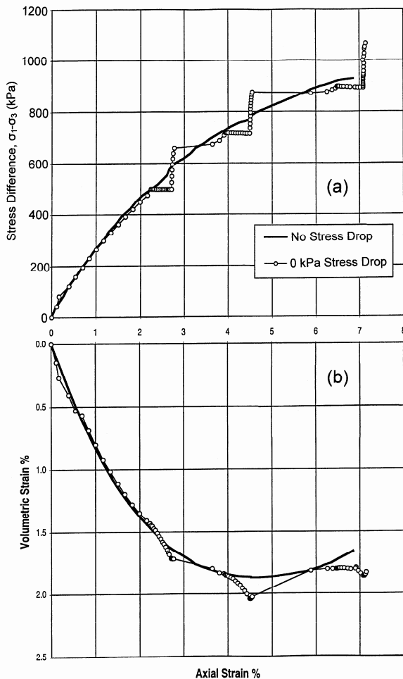
Figure 2. (a) Stress-strain and (b) volume change relations from load controlled drained triaxial compression test on crushed coral sand with creep stages of 1440 min. at stress differences of 500, 700, and 900 kPa. Comparison with results from load controlled test without creep stages.
