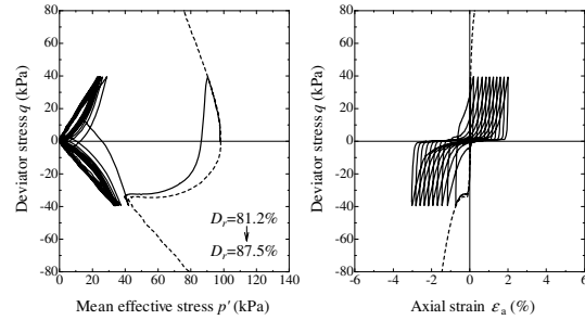
(d) In the case where the first cyclic undrained shear loading is halted at position equivalent to point [d] in Fig. 3
