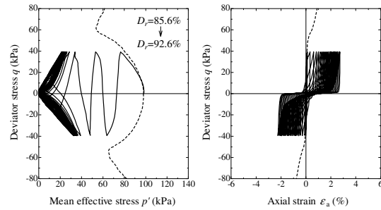
(c) In the case where the first cyclic undrained shear loading is halted at position equivalent to point [c] in Fig. 3
