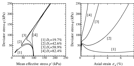
Figure 2. Monotonic compressive undrained shear behavior of sands with densities
