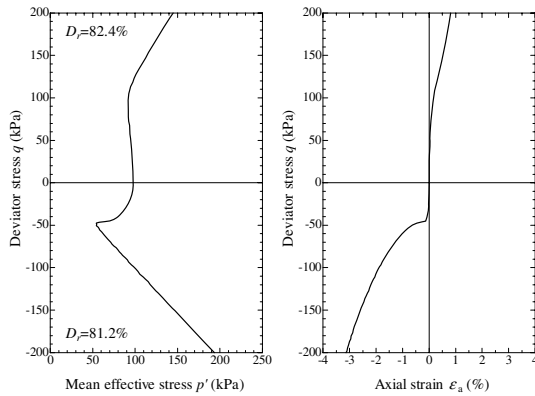
Figure 1. Monotonic undrained shear behavior of sand with initial anisotropy
