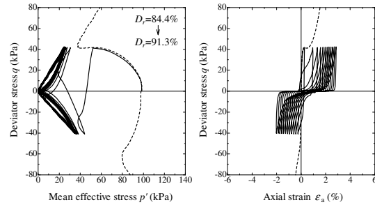
(b) In the case where the first cyclic undrained shear loading is halted at position equivalent to point [b] in Fig. 3
