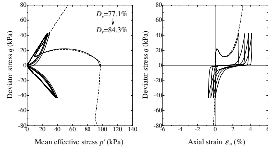
(a) In the case where the first cyclic undrained shear loading is halted at position equivalent to point [a] in Fig. 3
