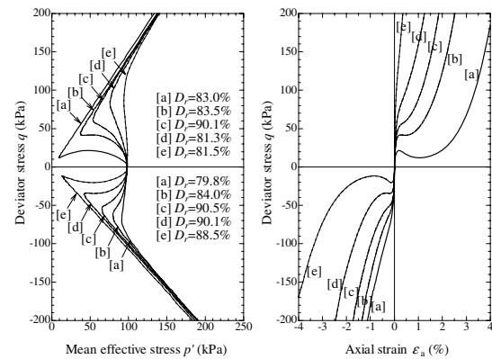
Figure 6. Monotonic undrained shear behavior of sand subjected to liquefaction history (In the case where cyclic undrained shear loading is halted at positions equivalent to points [a] to [e] in Fig. 3)
