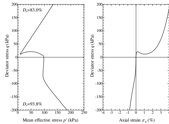
Figure 4. Monotonic undrained shear behavior of sand subjected to liquefaction history (In the case where cyclic undrained shear loading is halted at a position equivalent to point [a] in Fig. 3)
