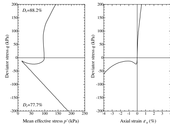
Figure 5. Monotonic undrained shear behavior of sand subjected to liquefaction history (In the case where cyclic undrained shear loading is halted at a position equivalent to point [f] in Fig. 3)
