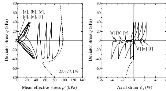
Figure 3. Cyclic undrained shear behavior of sand with initial anisotropy = liquefaction behavior
