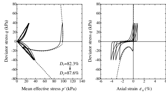
(e) In the case where the first cyclic undrained shear loading is halted at position equivalent to point [e] in Fig. 3
