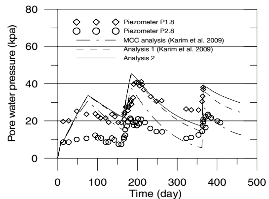
Figure 3. Excess pore water pressure response (field values and analysis results) at RL -4.5 m.
