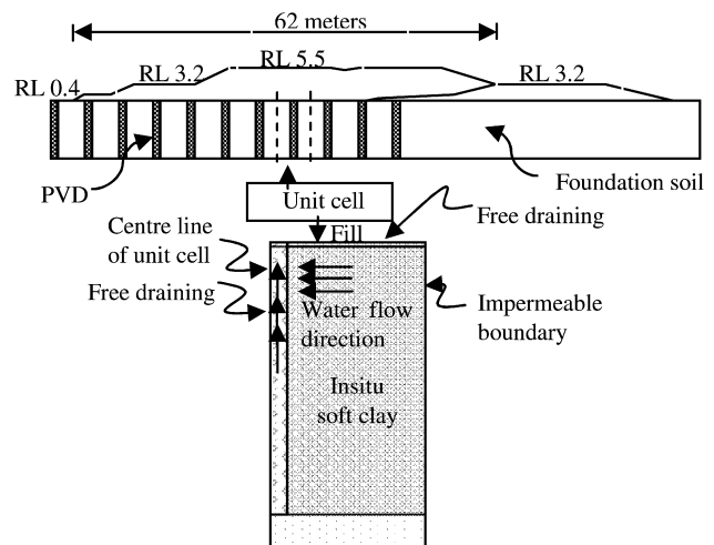
Figure 1. Transverse section of the embankment and the unitcell idealisation (not drawn according to scale).
