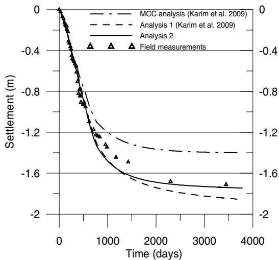
Figure 2. Time vs. settlement from three different analyses.
