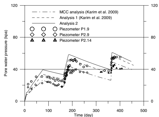
Figure 4. Excess pore water pressure response (field values and analysis results) at RL -7.5 m.
