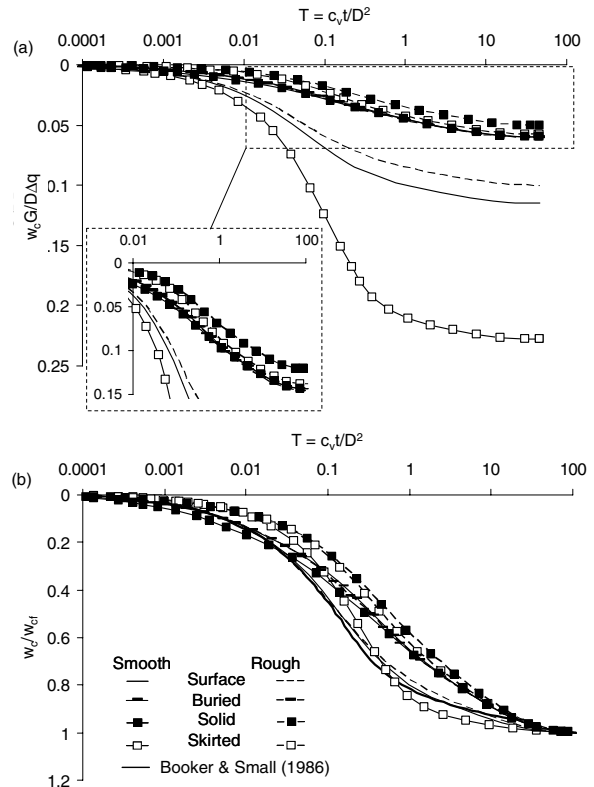
Figure 5. Settlement time histories
