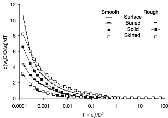
Figure 6. Rate of consolidation time histories
