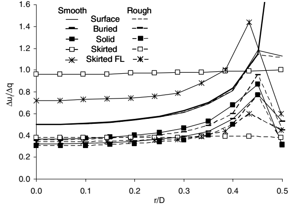
Figure 2. Initial contact pressures at foundation-soil interface
