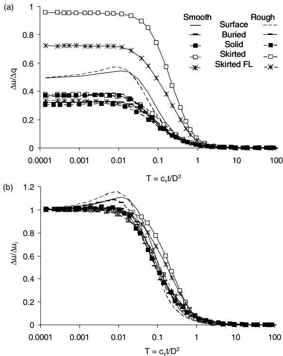
Figure 4. Excess pore pressure time histories
