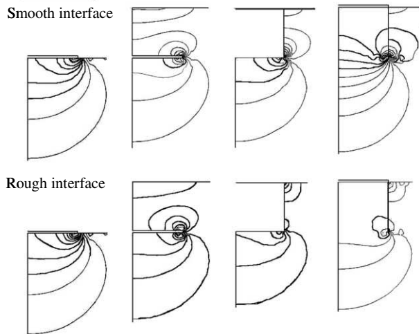
Figure 3. Initial excess pore pressure fields
