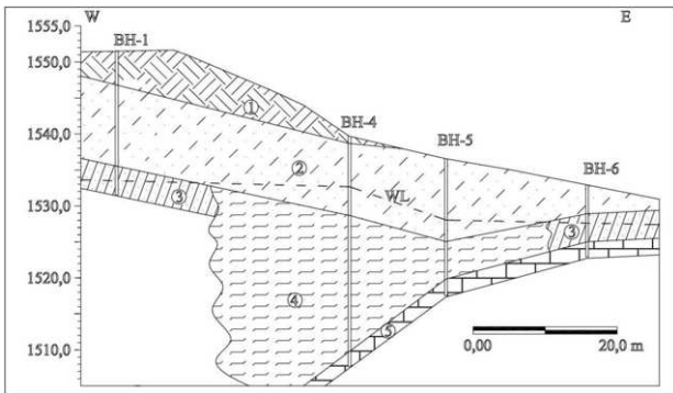
Fig. 4. Engineering geological profile 1 - embankment; 2 – sandy clay with single gravel pieces; 3 – gravelly sandy clay; 4 – weak zone of red-brown very soft sandy clay; 5 – marbles; WL - water level
