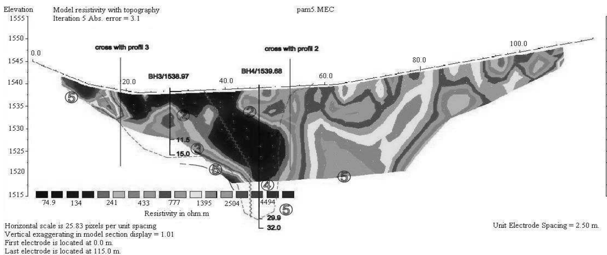
Fig. 5. Geophysical profile 2 – sandy clay; 3 – gravelly sandy clay; 4 – weak zone; 5 – marbles
