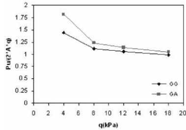
Figure 4. Variation of \mu against overburden pressure
