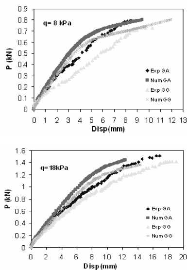
Figure 7. Comparison between numerical and experimental results for q = 8 and 18\text{ kPa}
