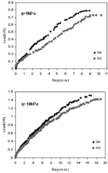
Figure 3. Comparison between behavior of geogrid and Grid-Anchor under 8 and 18 kPa
