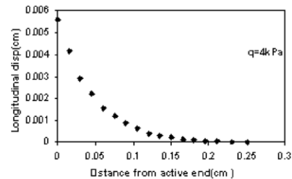
Figure 8. Grid – Anchor elongation during pull-out test by PLAXIS
