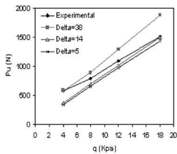
Figure 6. Comparison between analytical and experimental results
