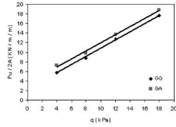
Figure 5. Relationship between ultimate pull-out stress ( P_u/2A ) and overburden pressure
