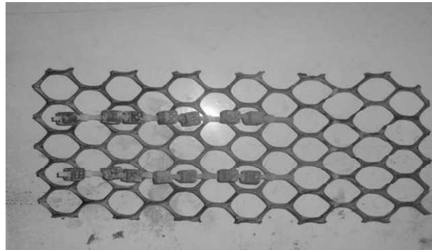
Figure 2. Grid – Anchor system
